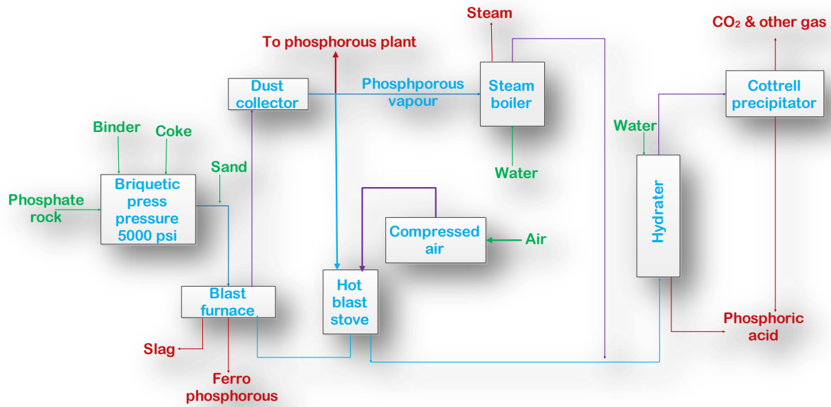
Figure: Manufacturing of Phosphoric acid using blast furnace
